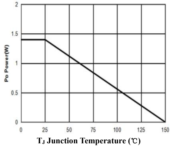
Figure 8: Power Dissipation
