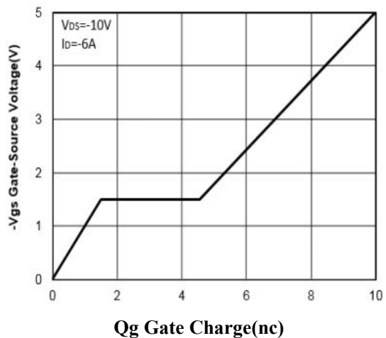
Figure 6: Gate-Charge Characteristics
