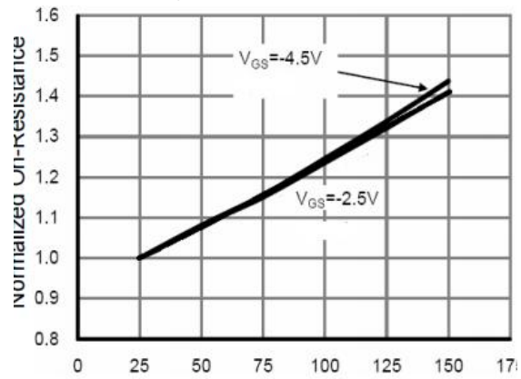
T_J Junction Temperature (°C) Figure 4: On-Resistance vs. Temperature
