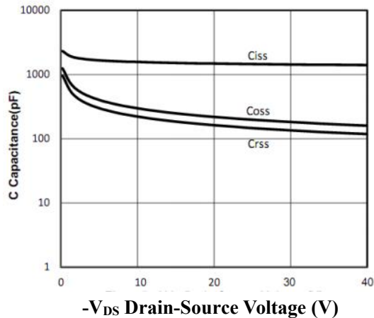
- V_{DS} Drain-Source Voltage (V) Figure 5: Capacitance Characteristics
