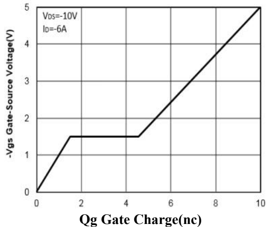
Q_g Gate Charge (nC) Figure 6: Gate-Charge Characteristics
