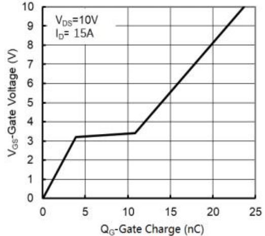
Figure 6: Gate-Charge Characteristics
