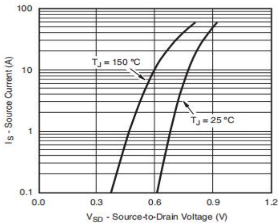
Figure 3: Diode Characteristics
