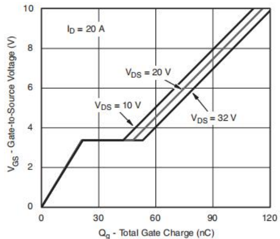
Figure 6: Gate-Charge Characteristics
