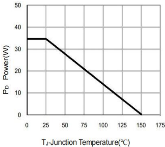
Figure 9: Power Dissipation
