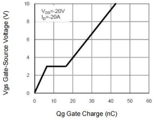
Figure 6: Gate-Charge Characteristics
