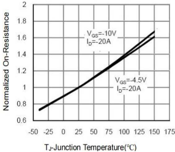
Figure 7: On-Resistance vs. Tj
