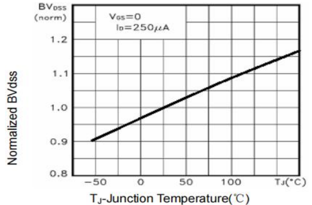
Figure 8: Breakdown Voltage vs. T_J
