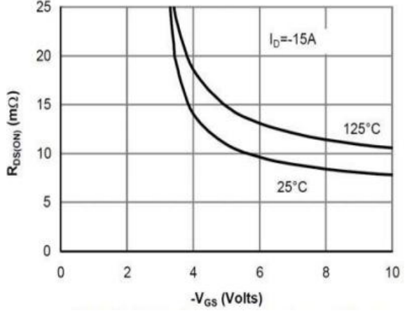
Figure 10: On-Resistance vs. Vgs
