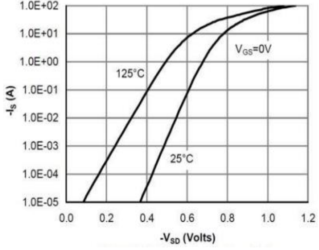
Figure 8: Diode Characteristics
