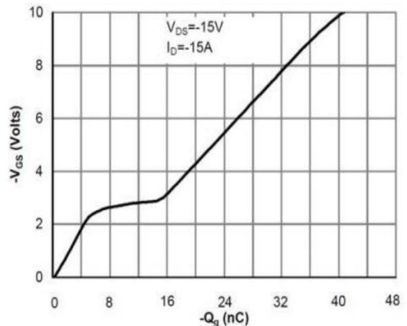
Figure 6: Gate-Charge Characteristics
