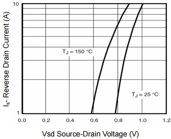
Figure 7: Diode Characteristics
