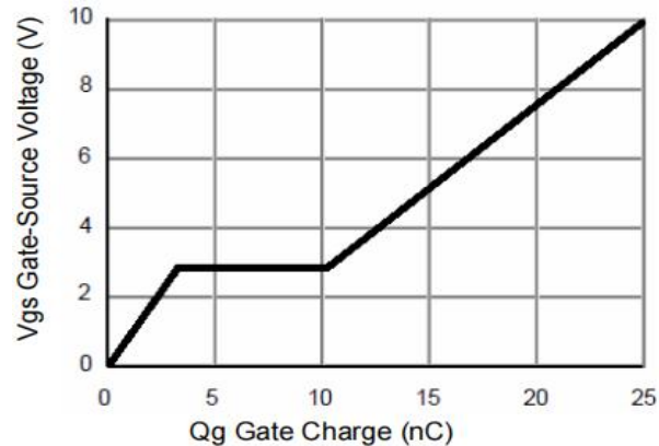
Figure 6: Gate-Charge Characteristics
