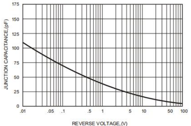
FIG.6-TYPICAL JUNCTION CAPACITANCE
