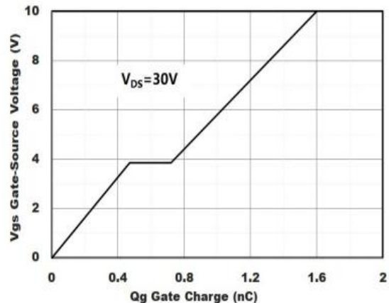
Figure 6: Gate-Charge Characteristics
