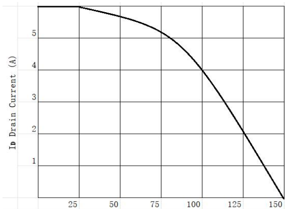
T J Junction Temperature (°C) Figure 7: Drain Current vs. Temperature
